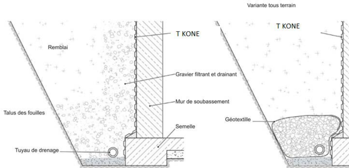
Figure 7 - Drainage
